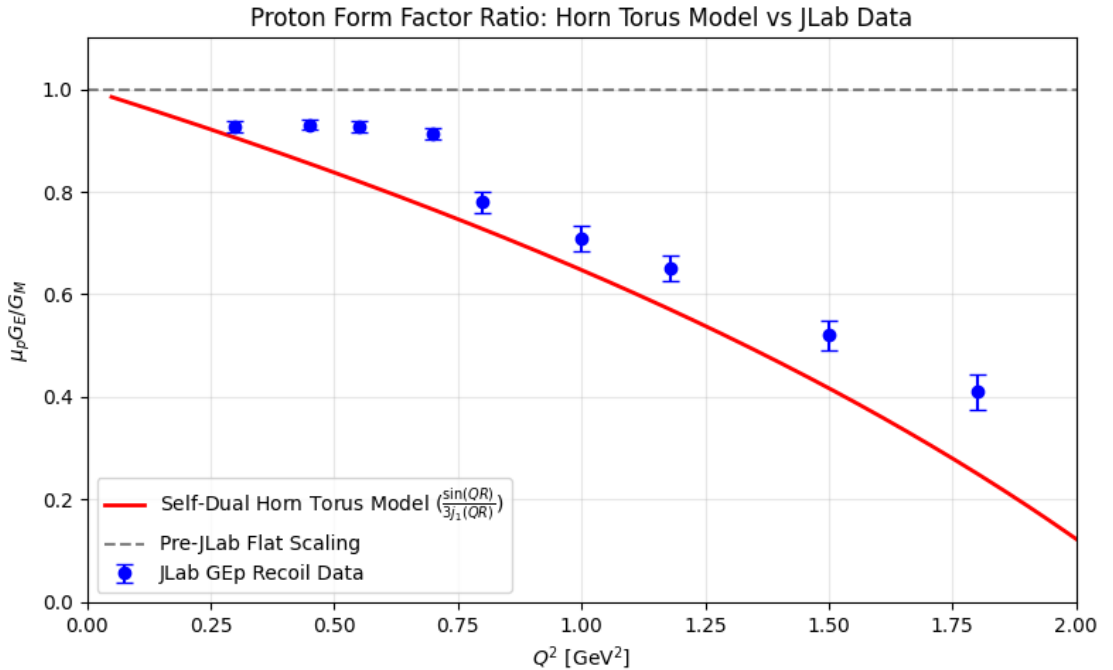
Figure 4: Comparison of the parameter-free 2D surface-integrated horn torus form factor ratio F_E(Q^2) against Jefferson Lab GEp recoil polarization data. Surface integration smooths classical diffraction nulls and eliminates unintegrated line poles, tracking the empirical drop-off without free variables.
