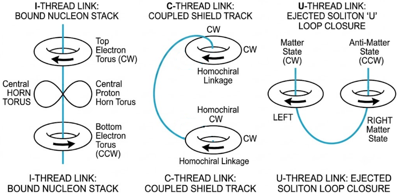
Figure 3: The ICU Topological Pair Genesis Taxonomy: (I) Inter-species Baryon-Lepton coupling forming a bound nucleon stack. (C) Homochiral Intra-species entanglement (Baryon-Baryon or Lepton-Lepton) linked by a subterranean Falaco thread. (U) Heterochiral Matter-Antimatter pair production born from the bifurcation of a sheared U-loop mesocyclone base.
