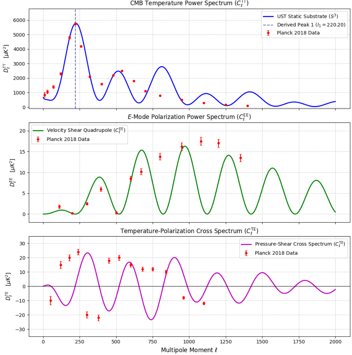
Figure 1: Angular power spectra ( C_l^{TT} , C_l^{EE} , C_l^{TE} ) calculated strictly under the static, non-expanding S^3 spatial substrate model overlaid with Planck 2018 observational data points. Top: Scalar temperature spectrum ( C_l^{TT} ) anchored by the double-cover node volume scale l_1 = 220.20 . Middle: E -mode polarization spectrum ( C_l^{EE} ) driven by quadrupolar velocity shear gradients ( \pi_{ij} \propto \nabla v ), naturally peaking near l \approx 1000 . Bottom: Coherent pressure-shear cross-correlation spectrum ( C_l^{TE} ).
