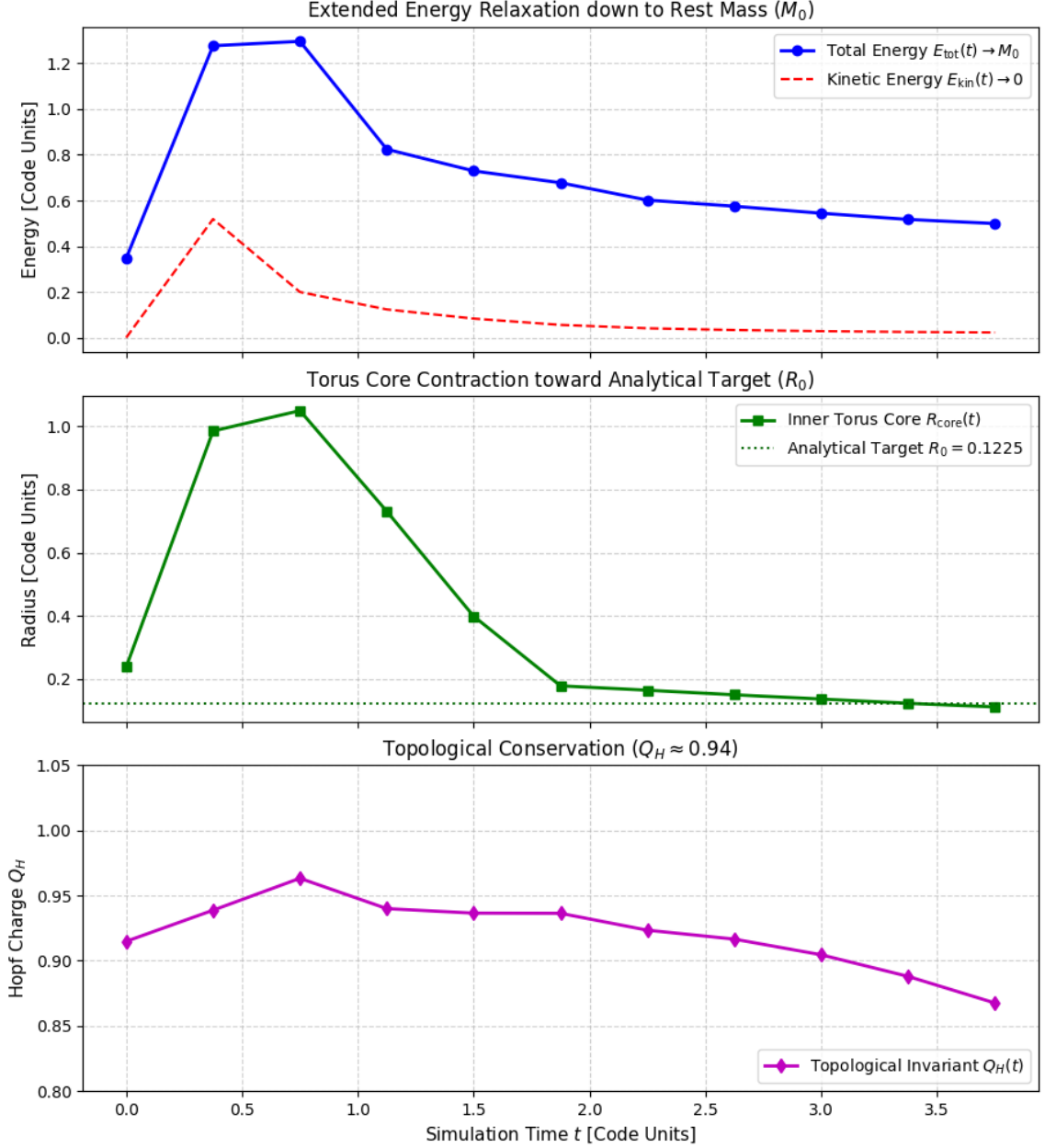
Figure 2: Numerical relaxation trajectory of the 3D Skyrme-Faddeev Q_H = 1 Hopfion knot soliton on an N = 64^3 spatial grid. Top: Total field energy E_{\text{tot}} relaxing toward the static rest-mass eigensolution M_0 as kinetic wave jitter dissipates ( E_{\text{kin}} \rightarrow 0 ). Middle: Inner torus core radius R_{\text{core}} contracting cleanly onto the analytical Hobart-Derrick equilibrium target R_0 = \sqrt{1.5}D_\gamma = 0.1225 code units. Bottom: Strict topological invariant protection ( Q_H \approx 0.94 ).
